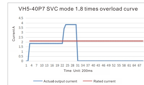
VH5 frequency converter 1.8 times overload time 1 second
