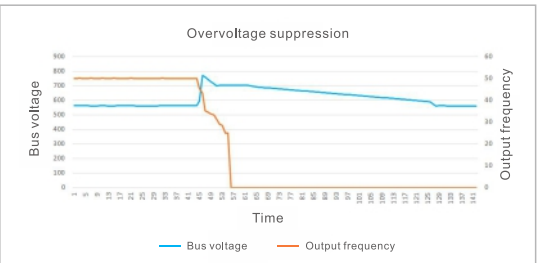
Overvoltage suppression is that when the bus voltage reaches or exceeds the bus overvoltage suppression point, the frequency converter will automatically adjust the operation frequency to suppress the rise of bus voltage, so as to ensure that the frequency converter will not cause overvoltage protection due to high bus voltage.
