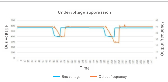
Undervoltage suppression is that when the bus voltage drops to the bus undervoltage suppression point, the frequency converter will automatically adjust the operation frequency, so as to ensure that the frequency converter will not report undervoltage fault due to low bus voltage in a short time. Once the power supply is restored within the validity period of undervoltage suppression, the frequency converter can continue to operate normally.
